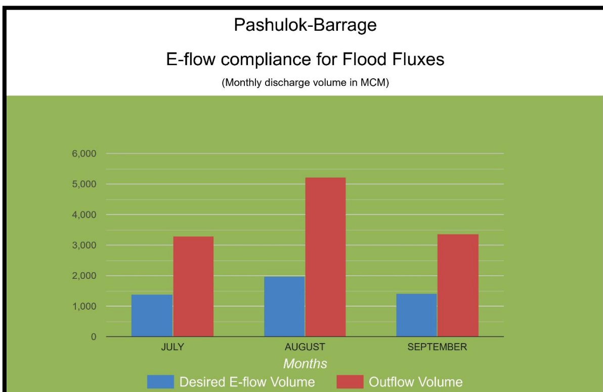
Figure 8: Graphs showing status of implementation of E-Flow at Pashulok Barrage
