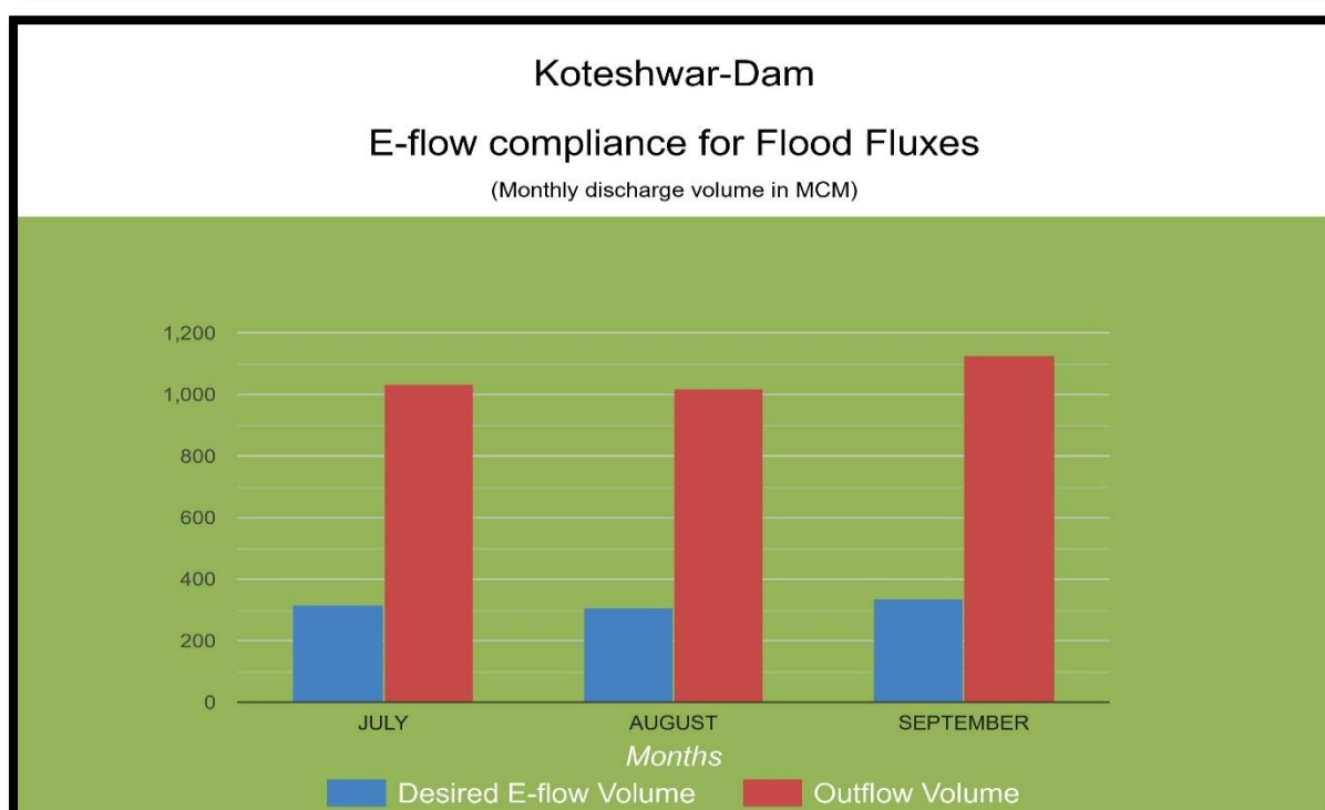
Figure 4: Graphs showing status of implementation of E-Flow at Tehri – Koteswar
