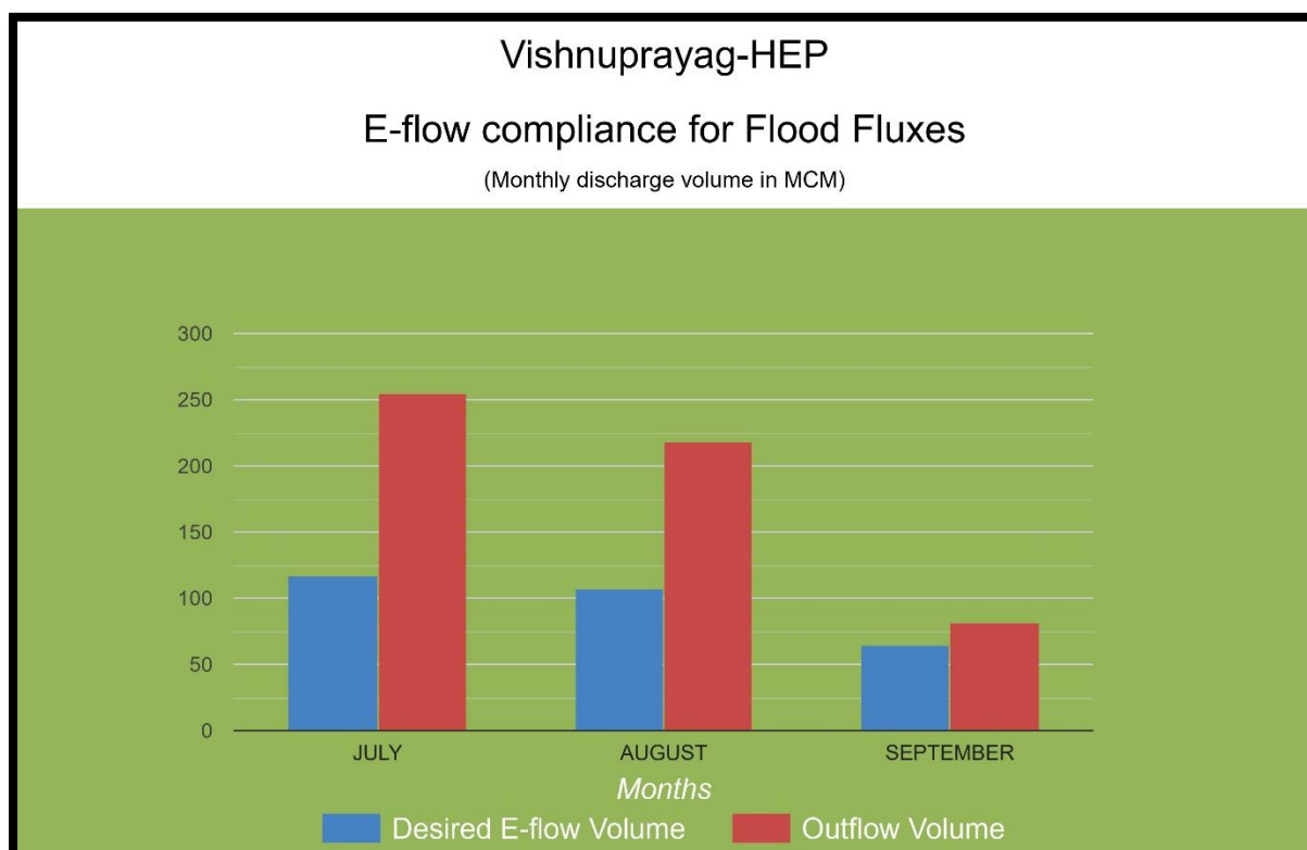
Figure 5: Graphs showing status of implementation of E-Flow at Vishnuprayag HEP
