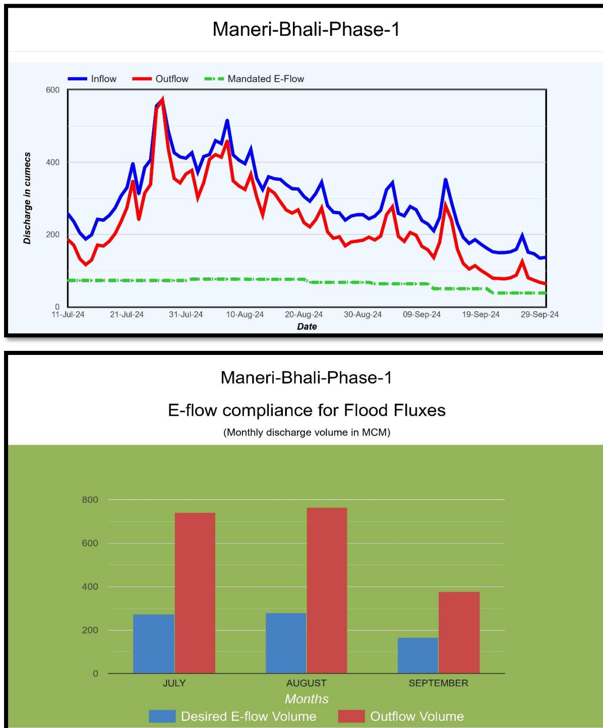
Figure 2: Graphs showing status of implementation of E-Flow at Maneri Bhali-I Project.
